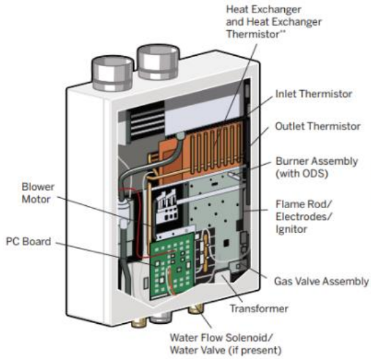
TANKLESS WATER HEATER
