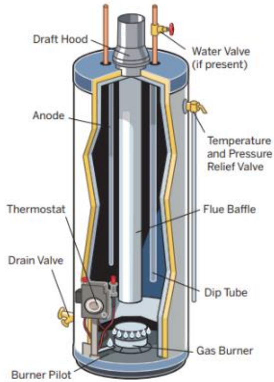
GAS WATER HEATER
